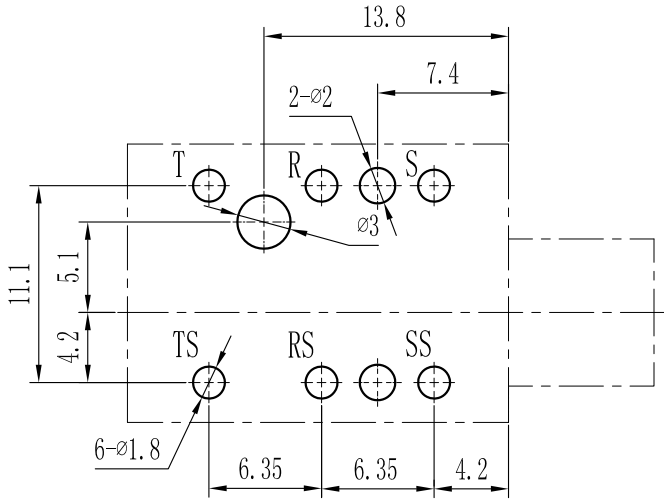
P.C.B LAYOUT (BOTTOM VIEW) Tolerance: \pm 0.05
