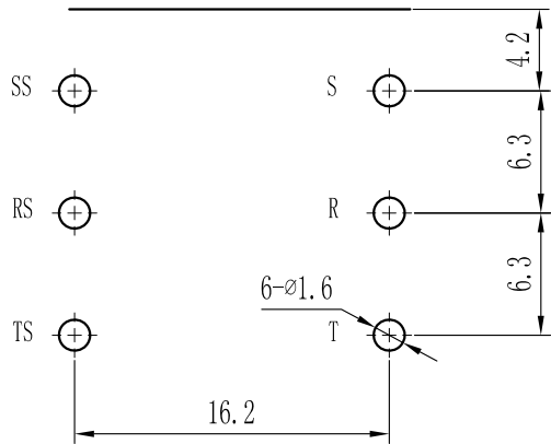
P.C.B LAYOUT (BOTTOM VIEW) Tolerance: ±0.05
