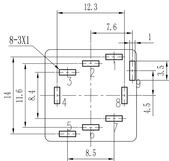
P.C.B LAYOUT (BOTTOM VIEW) Tolerance: \pm 0.05
