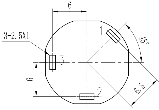
P. C. B LAYOUT (BOTTOM VIEW) Tolerance: ±0.05
