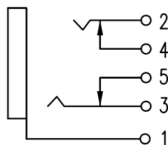
Electrical schematic
