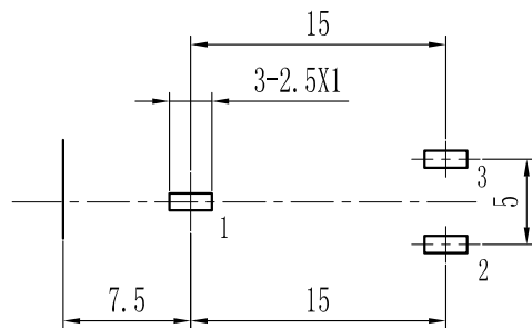
P.C.B LAYOUT (TOP VIEW) Tolerance: ±0.05
