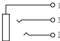
Electrical schematic
