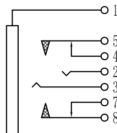
Electrical schematic
