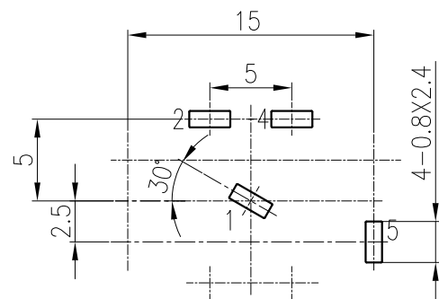
P. C. B LAYOUT (BOTTOM VIEW) Tolerance: ±0.05
